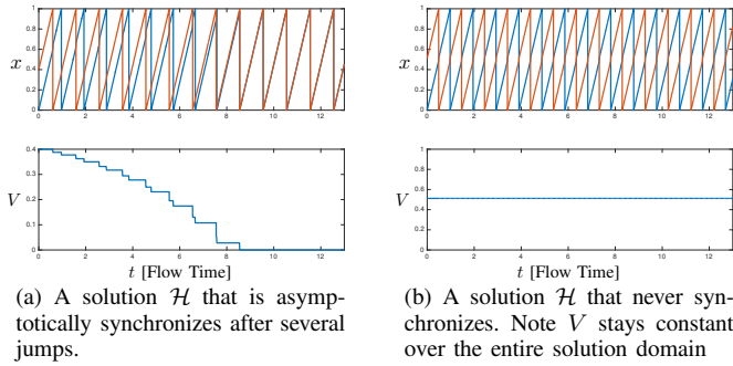
Fig. 2: Examples of solutions to \mathcal{H} for the impulse-coupled oscillator with \gamma(s) = \varepsilon s^2 , T = 1 , and \varepsilon = 0.1 . The function V over the respective solution is also given.
