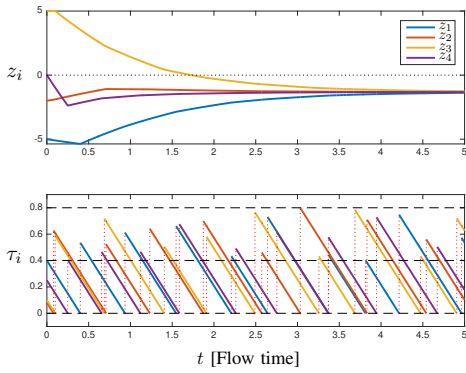
Fig. 1: The z, \tau components of a solution \phi = (\phi_z, \phi_\eta, \phi_\tau) to a hybrid system with agent dynamics (10), communication governed by local timers \tau_i with dynamics in (11), and distributed controller (12) and (13).
